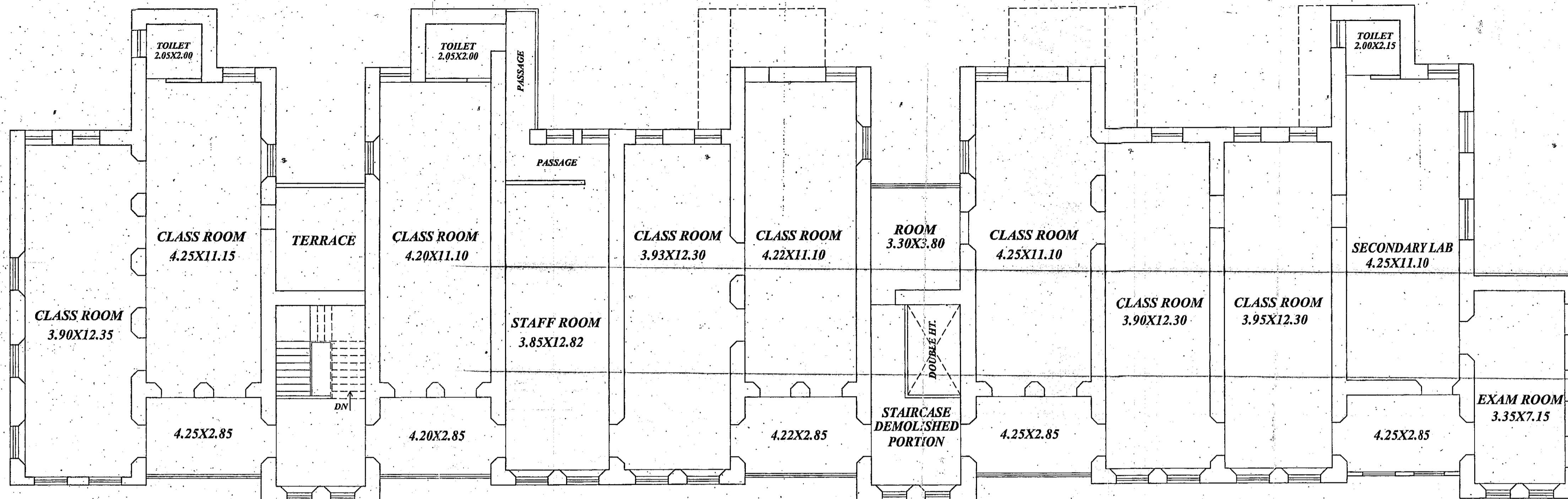
EXISTING FIRST FLOOR PLAN (BLDG. TYPE - B) SCALE : 1:100
