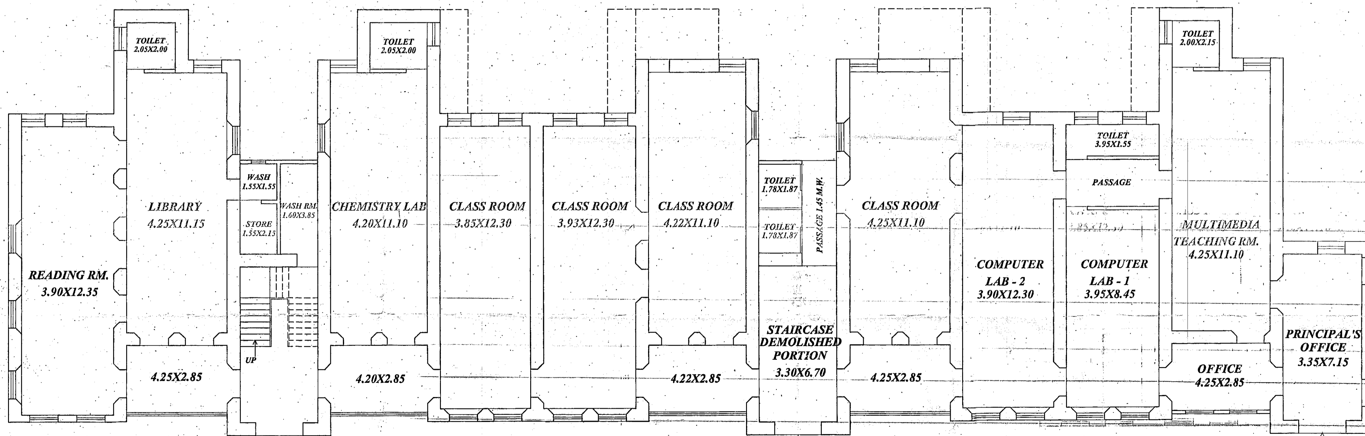
EXISTING GROUND FLOOR PLAN (BLDG. TYPE - B) SCALE : 1:100
